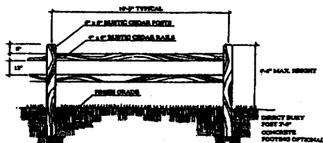
TYPICAL RUSTIC SPLIT RAIL FENCE NOT TO SCALE
