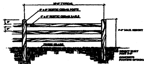
TYPICAL RUSTIC (3) RAIL FENCE NOT TO SCALE
